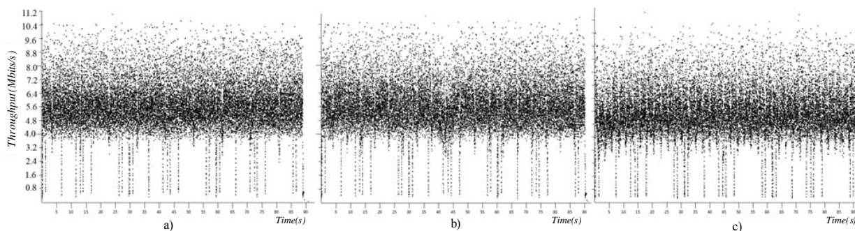
Fig. 7 Scenario 3 at the Rx-side with a transmission of 60MB with t_{IT} of a) 10sg, b) 5sg and c) 2.5sg
