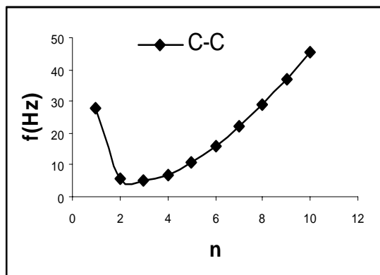
Fig. 2 Natural frequencies FG cylindrical shell associated with C-C boundary conditions. ( m=1 , h/R=0.002 , L/R=20 )
