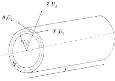
Fig. 1 Geometry of FGM cylindrical shell
