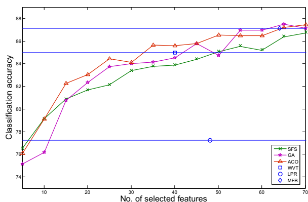
Fig1. Performance of feature selection methods
