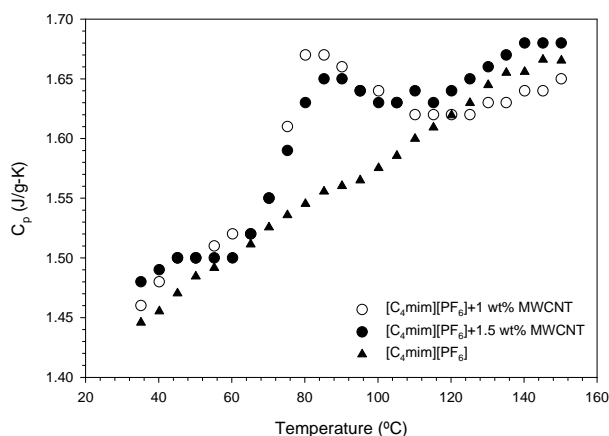
Fig. 5 Temperature-dependent heat capacity of CNT ionanofluids [12]
