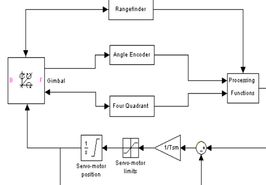
Fig. 1 The tracking system configuration
