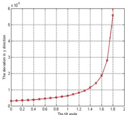
Fig. 3 The detector theory response to the input radiation angel
