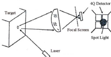
Fig. 2 The tracking sensor part schematic
