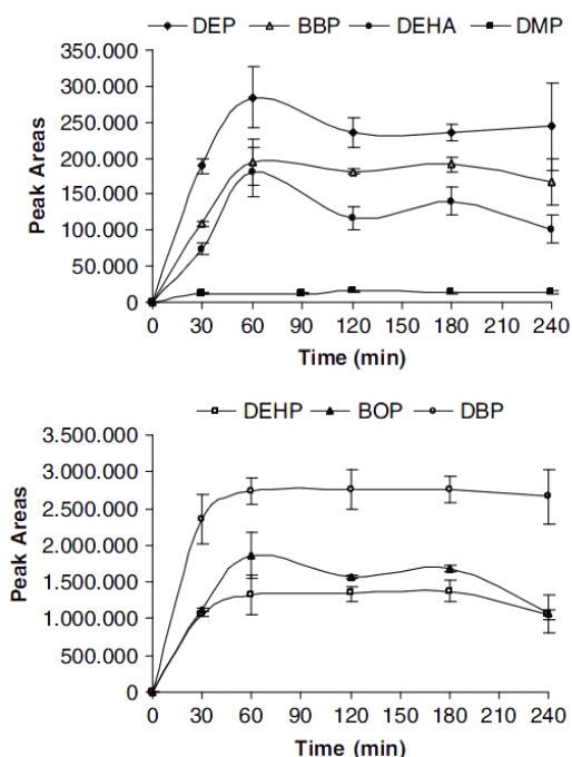
Fig. 2 Equilibrium-time profiles for the seven phthalates by SBSE-LD/LVI-GC-MS(SIM) at the 0.40 \mu\text{g/L} level (1000 rpm; LD solvent: MeOH) [23]
