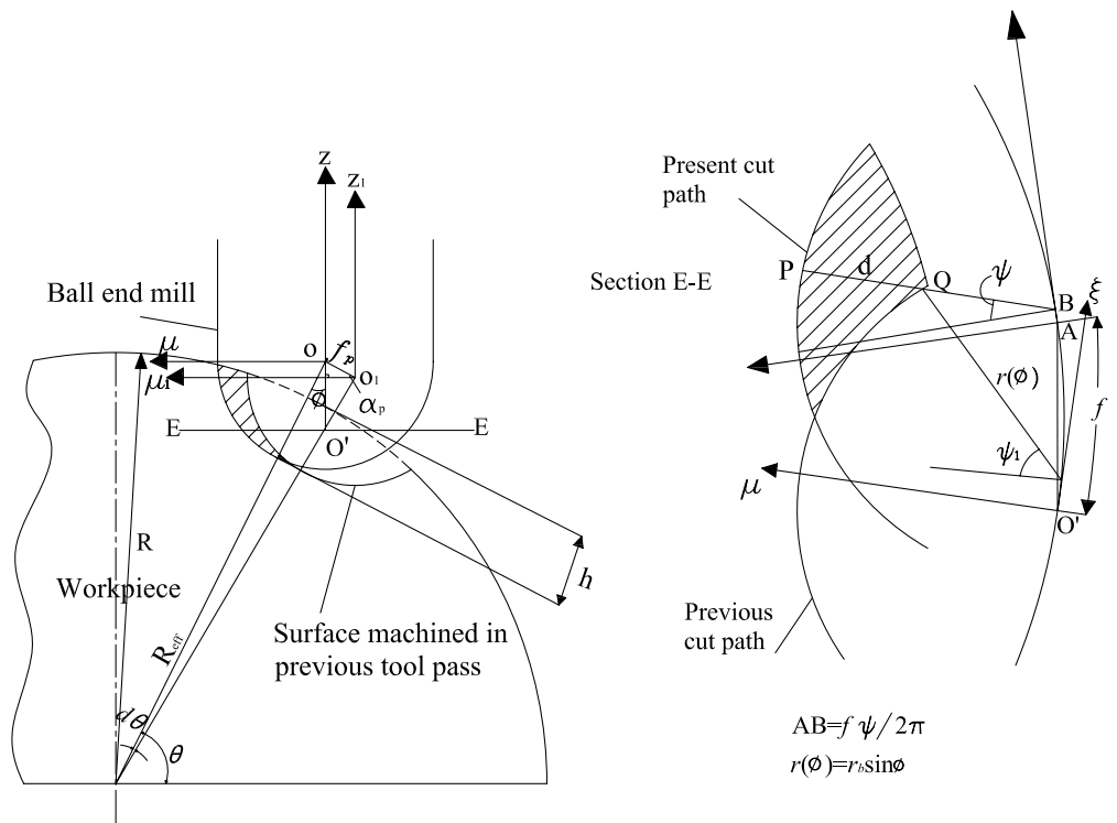
(a) Contouring
