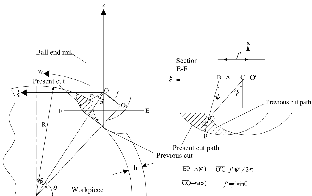
(b) ramping
