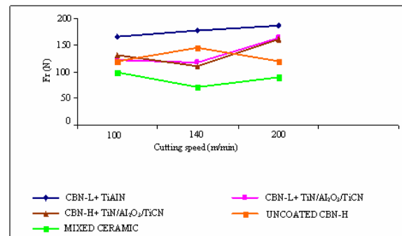
Fig. 3 Radial force and cutting speed relationship
