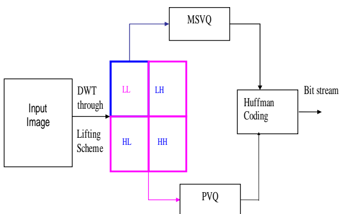
Fig. 5 Encoder of the Proposed Scheme
