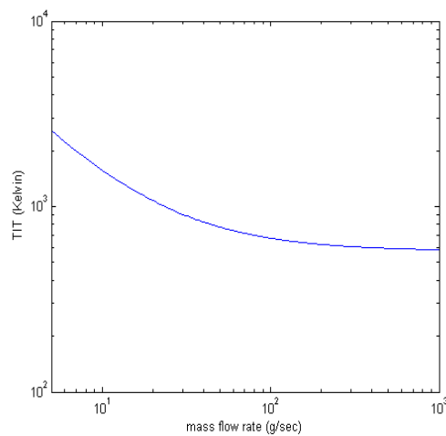
Fig. 26 Mass flow rate variation with turbine inlet temperature
