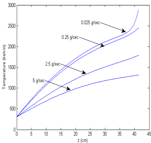
Fig. 15 Mass flow rate effect on fluid temperature
