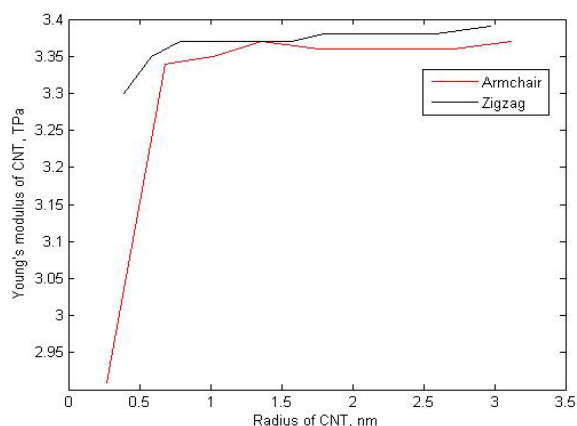
Fig. 2 Young's modulus vs radius of CNT
