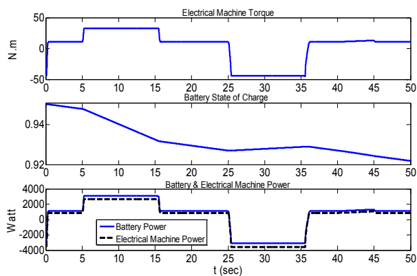
Fig. 22 Battery and electrical machine behavior
