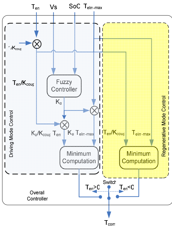
Fig. 14 Control strategy
