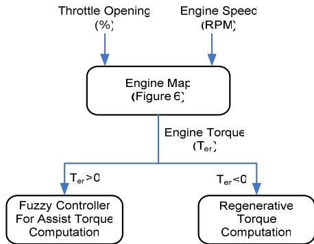
Fig. 13 Controller structure
