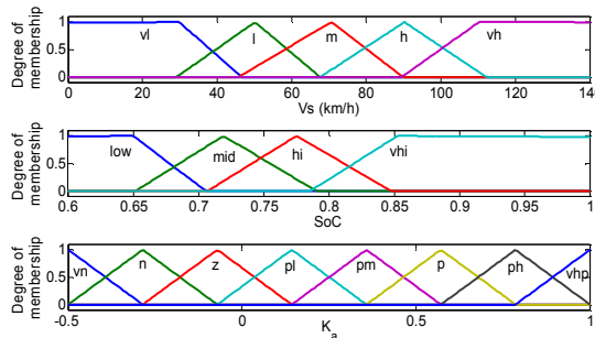
Fig. 15 Fuzzy controller memberships
