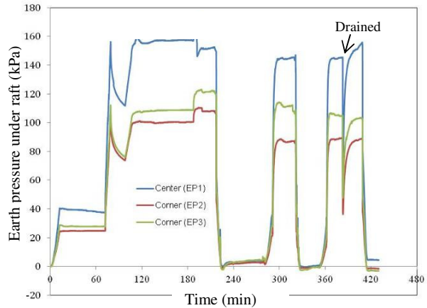
Fig. 23 Distribution of earth pressure under raft with time in case 1
