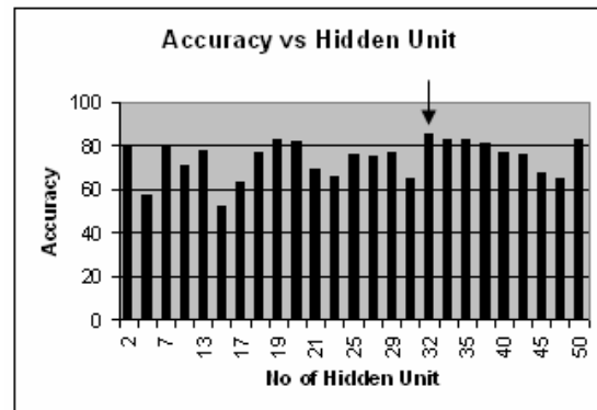
Fig. 5 Accuracy of the performance from different hidden units
