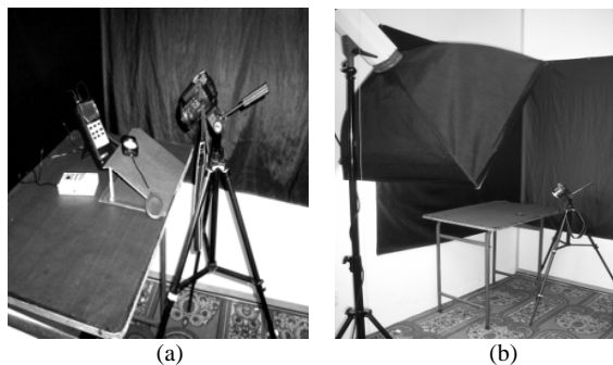
Fig. 3 The setting of capturing devices (a) camera placement, data logger and light meter placement (b) spotlight and table placement
