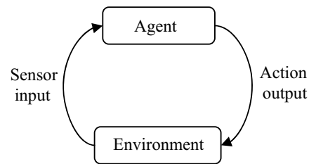
Fig. 1 Intelligent agent
