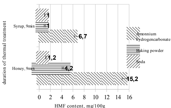
Fig. 7 Content of HMF in gingerbread biscuits baked at 200^{\circ}\text{C}
