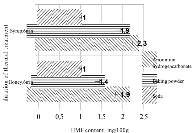
Fig. 6 Content of HMF in gingerbread biscuits baked at 200^{\circ}\text{C}
