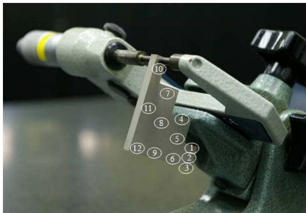
Fig. 6 Measurement position
