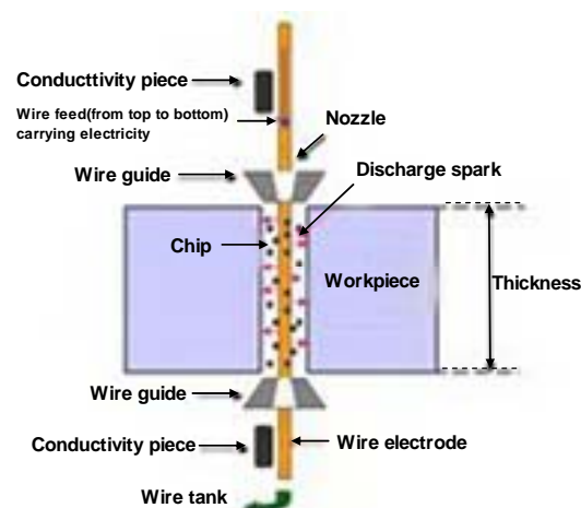
Fig. 1 Mechanism of Wire-cut EDM [1]
