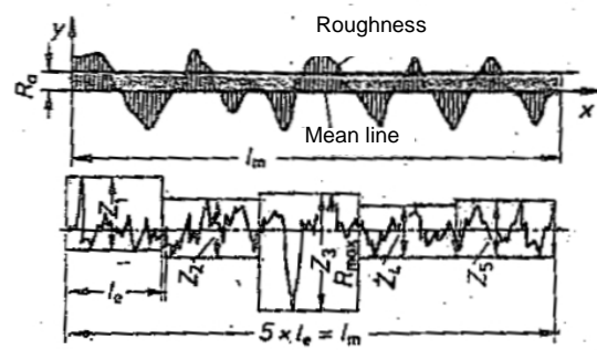
Fig. 4 Explain meaning of R_a , R_z and R_{max}
