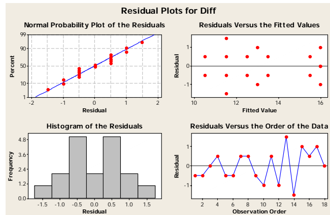
Fig. 12 Residual plot for cutting thickness error (Diff) in 2 nd section experiment
