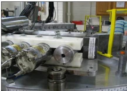
Fig. 2 Arrangement of laser beam system through adjustment with other detectors of tomography unit
