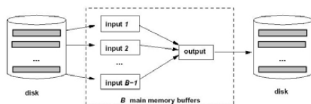
Fig. 1 General state of the external sorting
