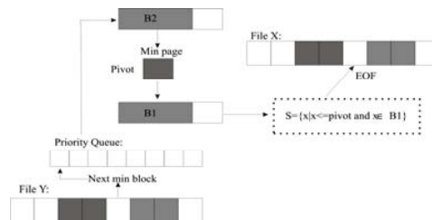
Fig. 2 New algorithm procedure
