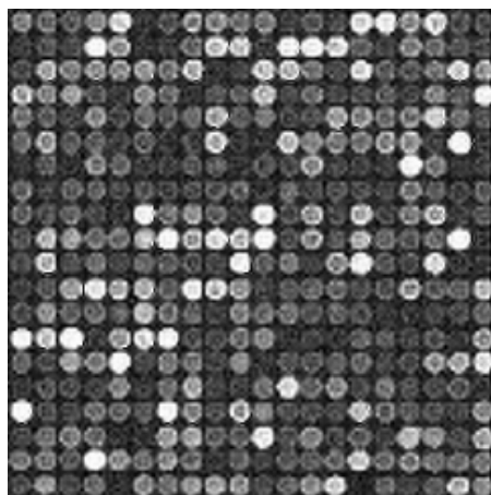
BayesShrink
