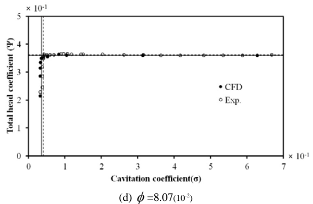
Fig. 8 Comparison with cavitation performance curve of experimental results and corrected numerical analysis
