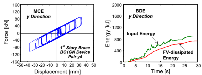
Fig. 15 Response cycles of most stressed BC1GN spring-damper pair, and energy time-histories in y direction obtained from the most demanding MCE and BDE-scaled input accelerogram, respectively
