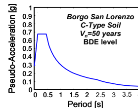
Fig. 13 Elastic response spectrum for Borgo San Lorenzo, BDE level, V_n=50 years, C_u=1 , topographic category T1, and C-type soil
