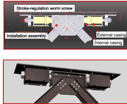
Fig. 12 Special installation layout of FV spring-dampers designed for the Borgo San Lorenzo building
