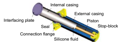
Fig. 2 Perspective cross section of a pressurized FV spring-damper
