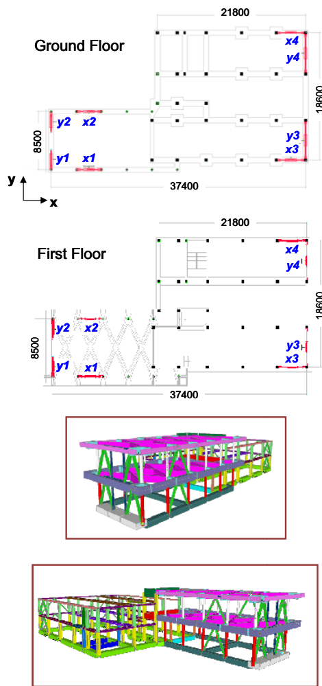
Fig. 11 Distribution of DB alignments in plan and elevation
