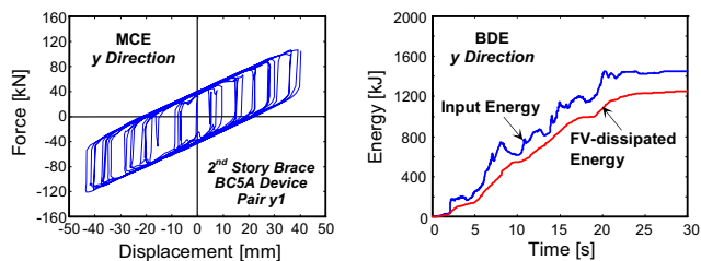
Fig. 7 Response cycles of most stressed BC5A spring-damper pair, and energy time-histories in y direction obtained from the most demanding MCE and BDE-scaled input accelerogram, respectively
