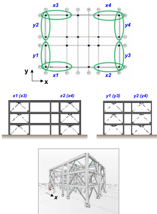
Fig. 3 Distribution of DB alignments in plan and elevation
