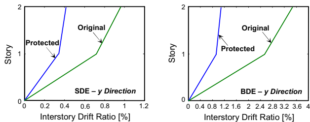
Fig. 14 Maximum interstory drift profiles in y direction (mean values)
