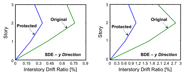
Fig. 6 Maximum interstory drift profiles in y direction (mean values)
