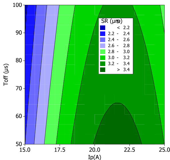
Fig. 4. Effect of I_p & T_{off} on SR
