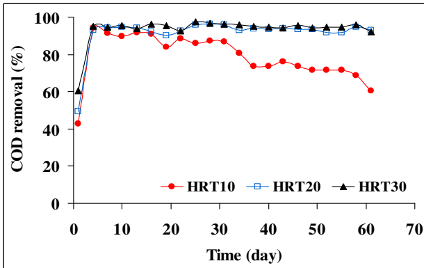
Fig. 9 COD removal at various hydraulic retention times
