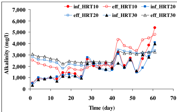
Fig. 5 Alkalinity during the CSTR operation
