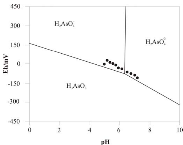
Fig. 3 The pH vs. Eh plot show only the presence of the \text{As}^{5+} in the groundwater
