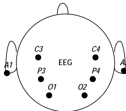
Fig. 1 Electrode placement
