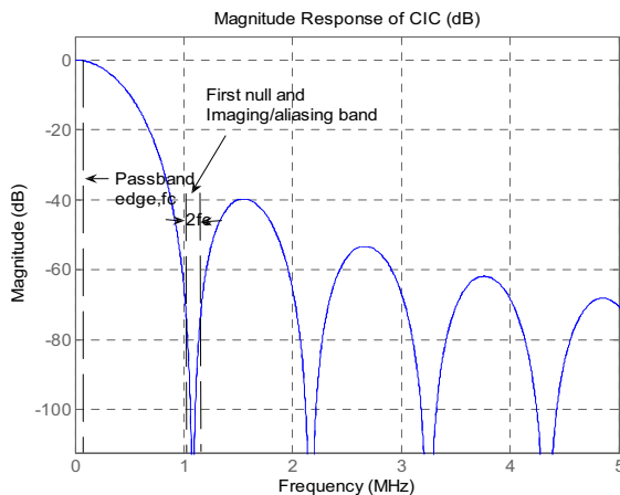
Fig. 4 CIC magnitude response for GSM with F_s = 34.667 MHz, R = 32 , M = 1 and k = 3
