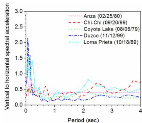
Fig. 5 Vertical to horizontal spectral acceleration
