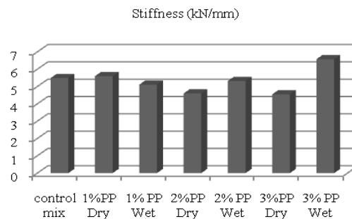
Fig. 5 Stiffness Vs Binder content for control, Wet and Dry PP Modified bitumrn
