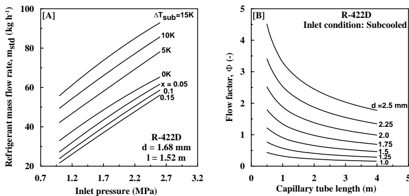
Fig. 5 Capillary tube rating charts for R-422D
