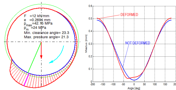
Fig. 5 Pressure distribution for JB1 configuration ( \alpha=0 , T_{in}=40^{\circ}\text{C} – T_{out}=80^{\circ}\text{C} ) with deformable components (left). Lubrication gap for rigid and deformable components (right)
