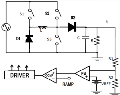
Fig. 4 Simulation circuit
