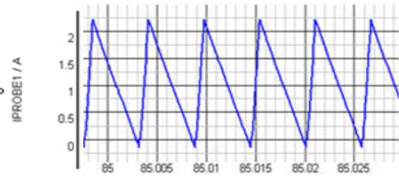
Fig. 20 Inductor current in BCM
