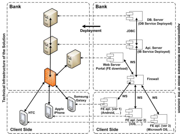
Fig. 2 Integration and Deployment Model [authors]
