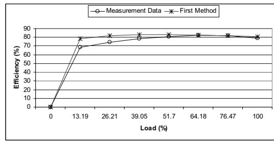
Fig. 2. Measured o and estimated * efficiency versus load in the first method, for the first motor
