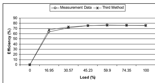
Fig. 8. Measured o and estimated e efficiency versus load in the third method, for the second motor
