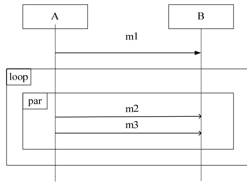
Fig. 3 An example of sequence diagram
