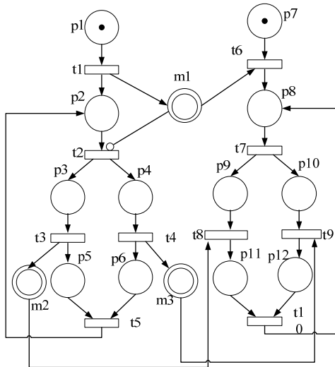
Fig. 6 Improved ECPN with synchronous messages transformed
