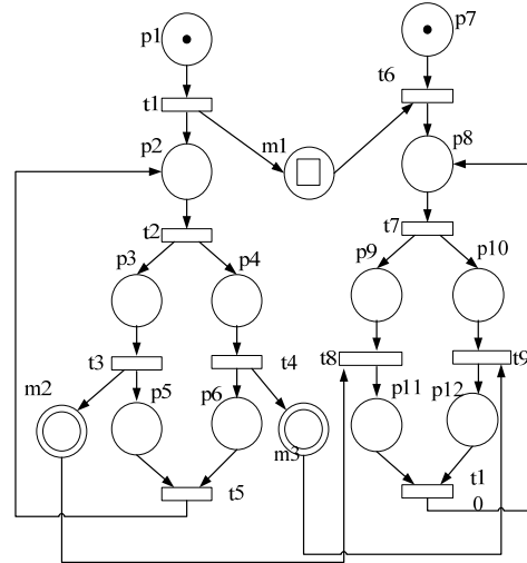
Fig. 5 Merging of ECPNs
