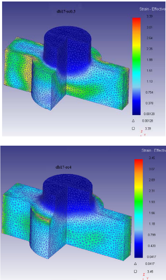
Fig. 17. The effective strain distribution in two die corner radius (rc=0.5 and rc=4mm)
