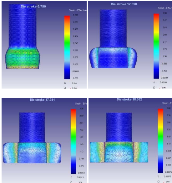
Fig. 13. Teeth formation stages for two teeth parts
