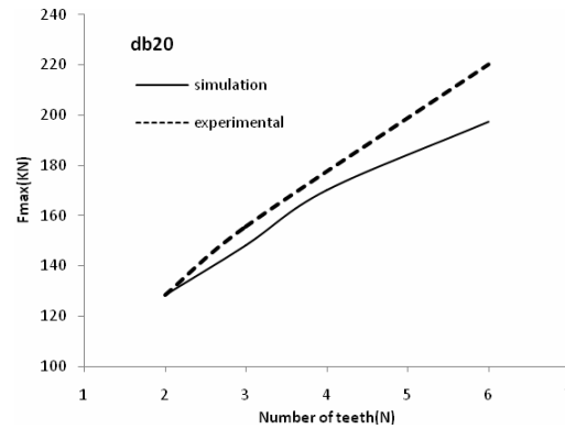
Fig. 11. Effect of teeth number on maximum forging load (db=20mm)
