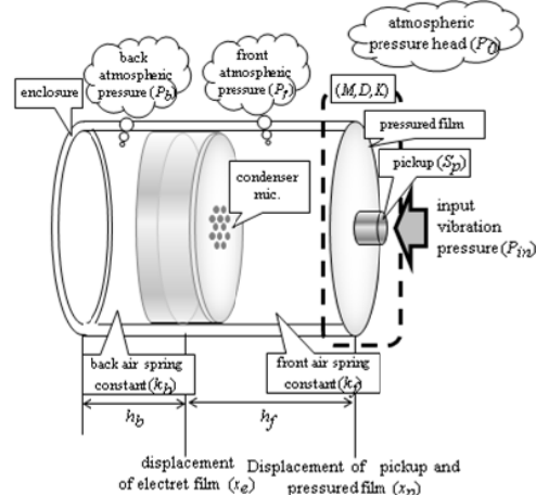
Fig. 3 Structure of an enclosed condenser microphone as vibration sensor
