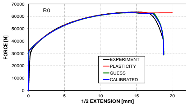
Fig. 9 Comparison of the experimental curve with calibrated curve – smooth sample
