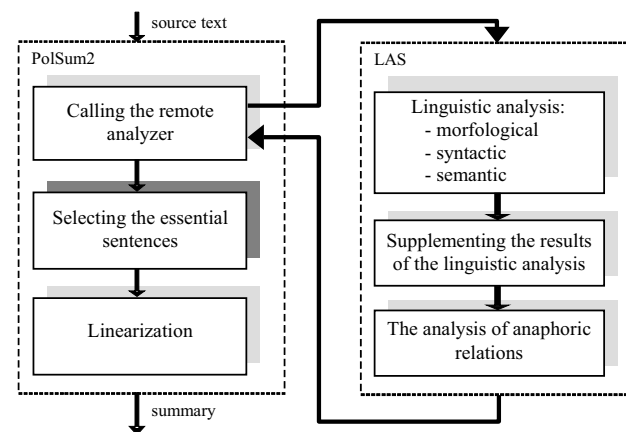
FIG. 1. THE STAGES OF SUMMARY GENERATION
