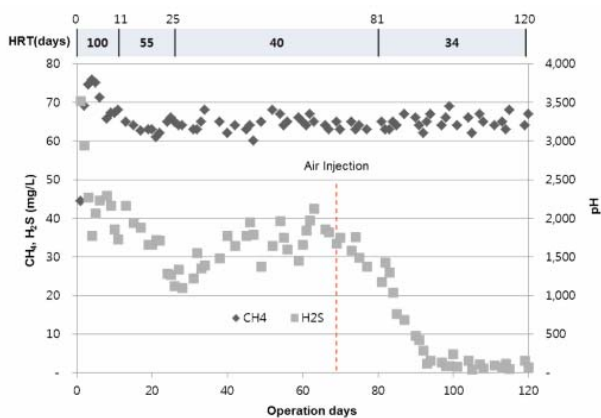
Fig. 6 Changes in methane and hydrogen sulfide concentrations
