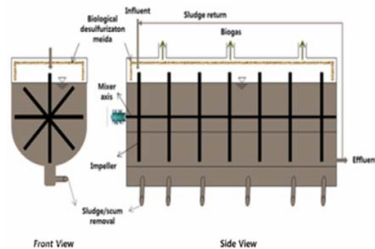
Fig. 1 Schematic diagram of the horizontal anaerobic digester
