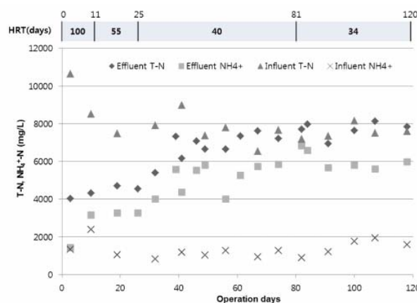
Fig. 5 Changes in concentrations of T-N and NH 4 + -N
