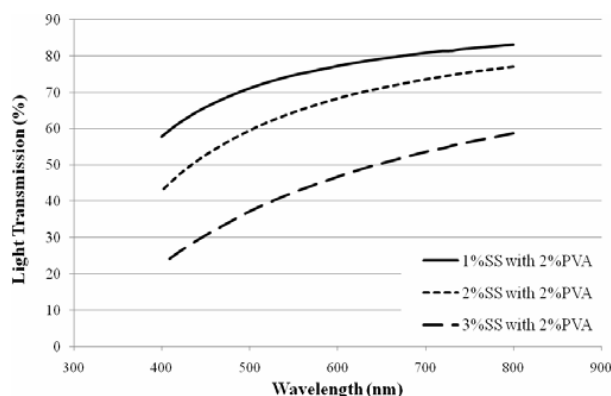
Fig. 2 Percentage of light transmission of SS films
