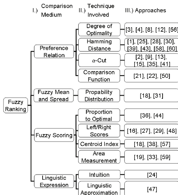
Fig. 1. A Taxonomy of Fuzzy Ranking Methods
