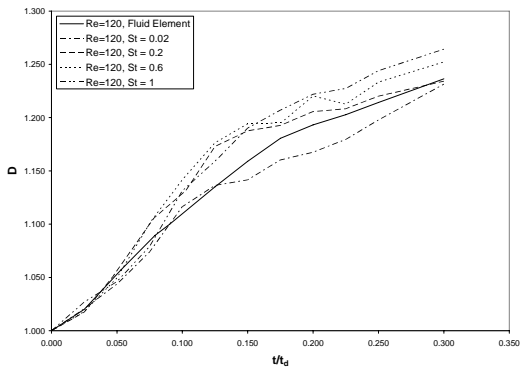
Fig. 2 Fractal dimension of heavy particle lines as a function of the normalized for k_N/k_I=36 and different Stokes numbers
