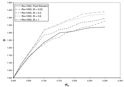
Fig. 6 Fractal dimension of heavy particle lines as a function of the normalized time for k_N/k_I=178 and different Stokes numbers
