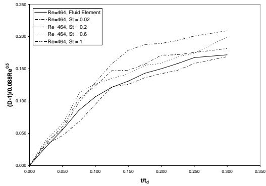
Fig. 5 Normalized fractal dimension of heavy particle lines as a function of the normalized time for k_N/k_I=100 and different Stokes numbers
