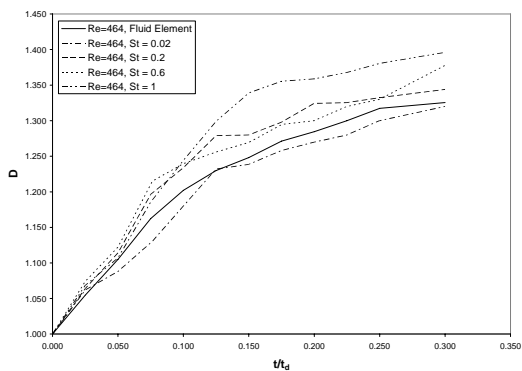
Fig. 4 Fractal dimension of heavy particle lines as a function of the normalized time for k_N/k_I=100 and different Stokes numbers
