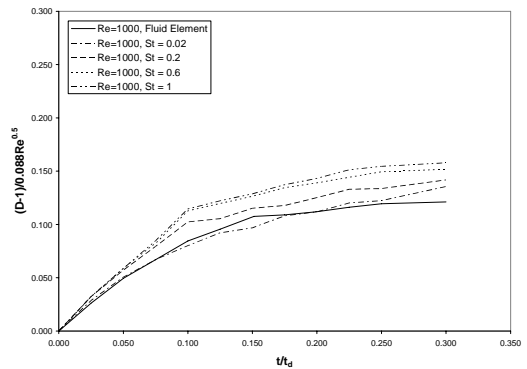
Fig. 7 Normalized fractal dimension of heavy particle lines as a function of the normalized time for k_N/k_I=178 and different Stokes numbers
