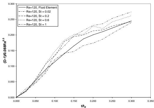
Fig. 3 Normalized fractal dimension of heavy particle lines as a function of the normalized time for k_N/k_I=36 and different Stokes numbers
