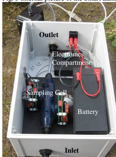
Fig. 3 Internal picture of the Smart Landfill Unit
