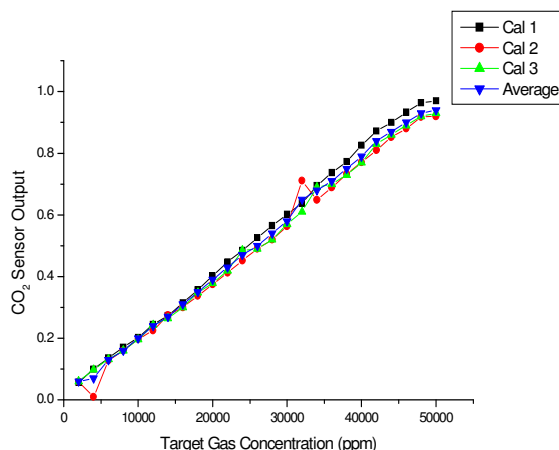
Fig. 1 Calibration data for IRCel CO 2 sensor
