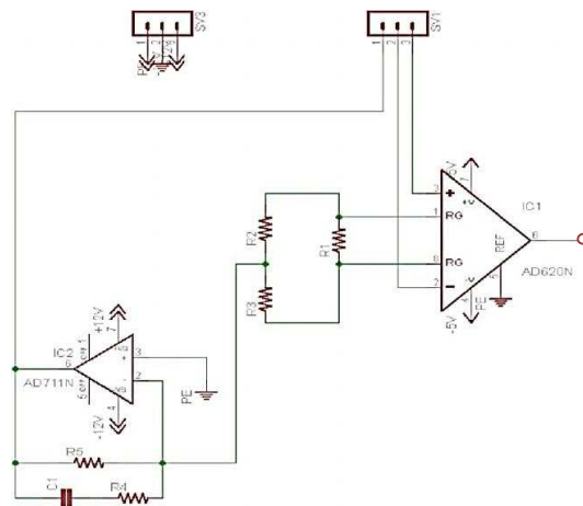
Fig. 2 Bio-Amplifier
