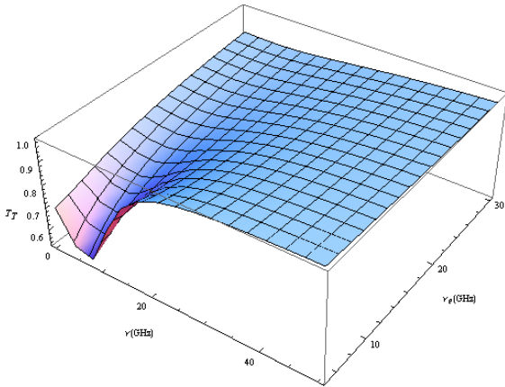
Fig. 6. Dependence of total transmitted power of hydrogen plasma slab in the presence of CNTs on microwave frequency for different value of \nu_c , where n = 2.181 \times 10^{17} m^{-3} and \nu_c = 5 GHz.
