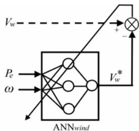
Fig. 4. Training scheme of ANN_{wind} .
