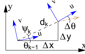
Fig. 2. Change in the robot pose as measured by the odometry system
