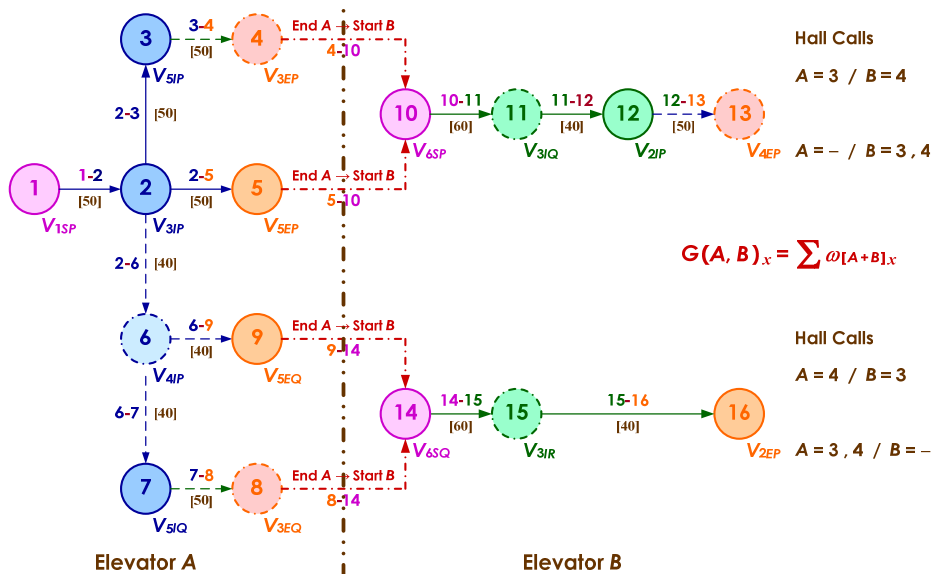
Fig. 6 Relabeled weighted graph for simulation software
