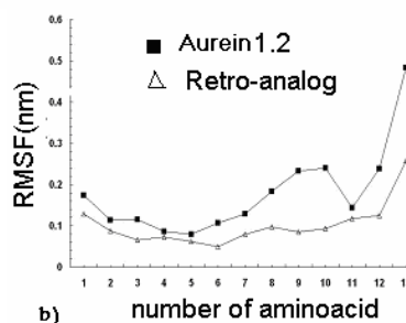
Fig. 2 (a) RMSDs versus time for the \text{C}_\alpha atoms in the two simulations: Aurein1.2 in TFE (gray line) and Retro-analog in TFE (black line) (b) RMSF from the initial minimized structure of aurein1.2 and retro-analog in TFE
